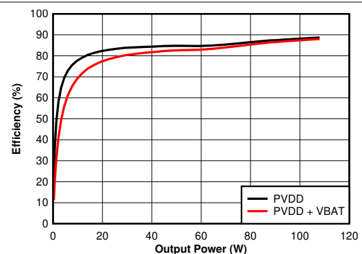
Figure 6-5. Efficiency vs Output Power - 4 \Omega
