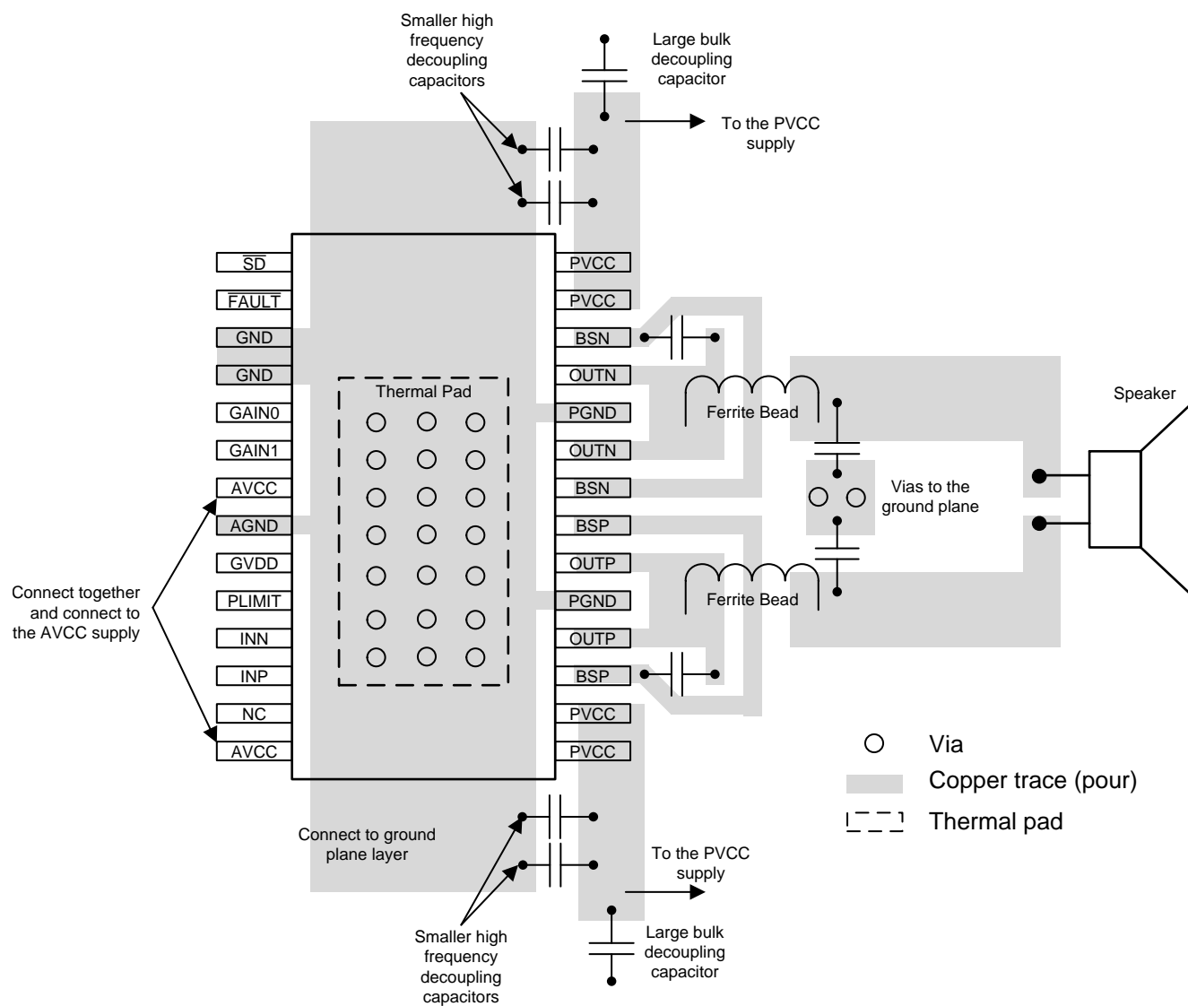
Figure 21. Recommended Layout
