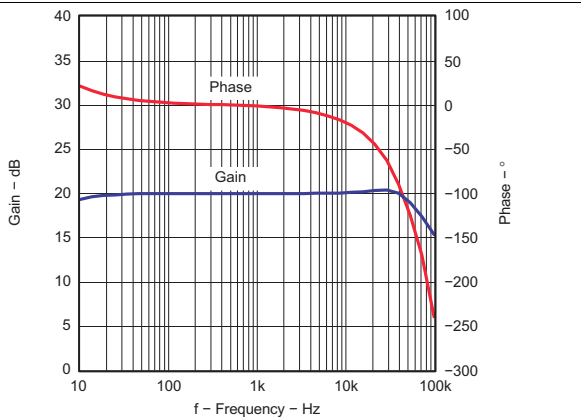
Gain = 20 dB V_{CC} = 12 V Z_L = 8 \Omega +66 \mu\text{H} C_1 = 1 \mu\text{F} V_I = 0.1 V RMS Filter = Audio Precision AUX-0025
