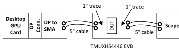
Figure 7-6. 8.1Gbps DP Compliance Setup - with TMUXHS4446
