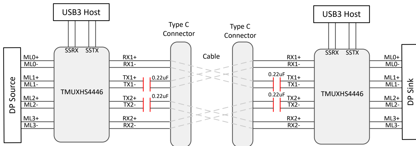
Figure 7-3. Typical Placement of AC Coupling Capacitors with V_{cm} \leq 1.8V
