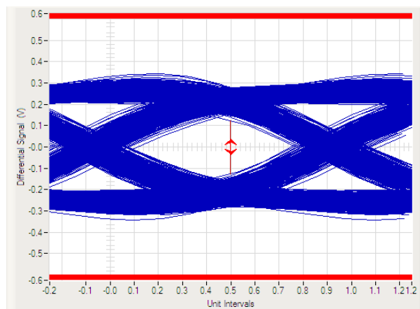
Figure 7-12. 10Gbps USB Compliance Eye Diagram - with TMUXHS4446
