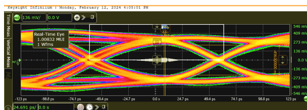
Figure 7-7. 8.1Gbps DP Compliance Eye Diagram - Baseline Setup (no DUT)
