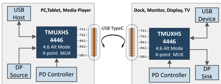
Figure 7-1. TMUXHS4446 in USB Type-C Source and Sink Applications
