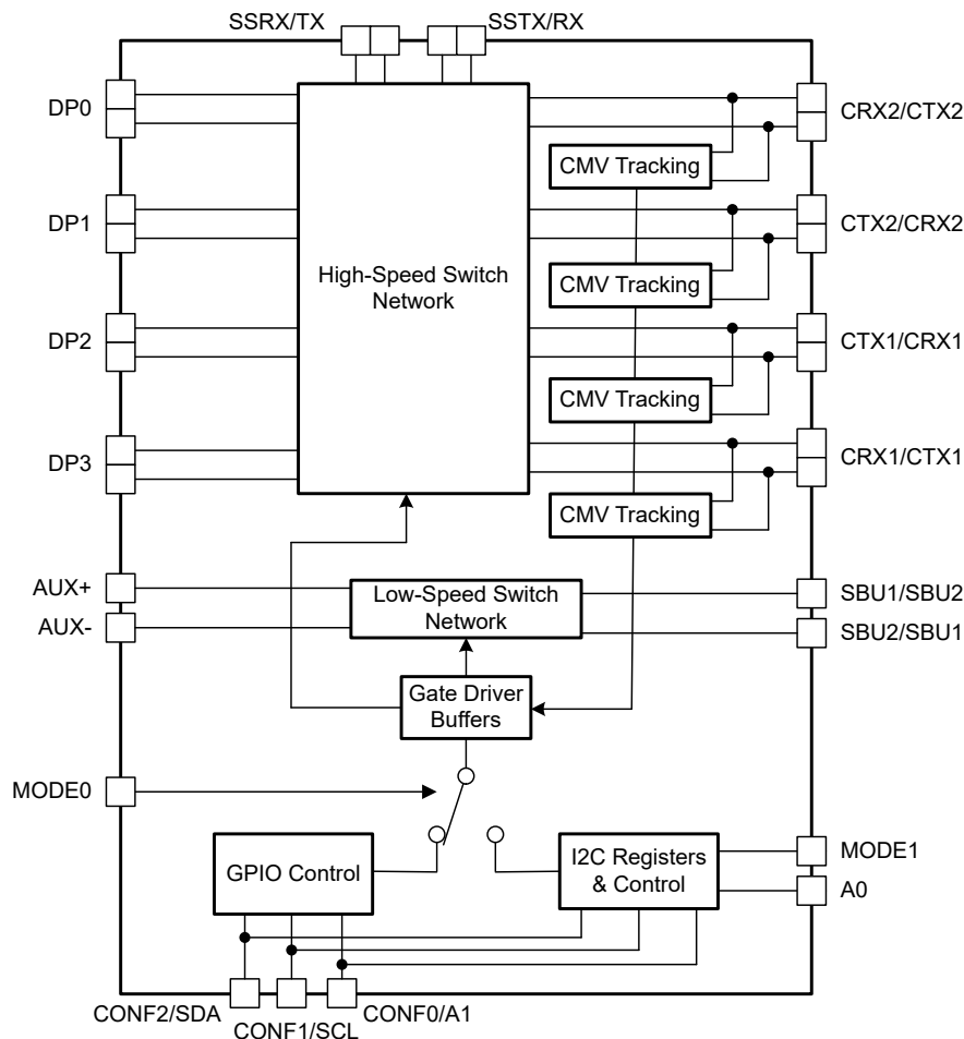
Figure 6-1. TMUXHS4446 Functional Block Diagram
