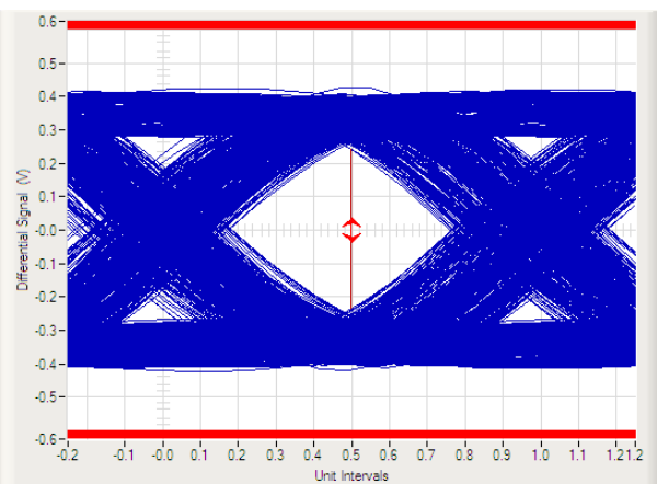
Figure 7-11. 10Gbps USB Compliance Eye Diagram - Baseline Setup (no DUT)
