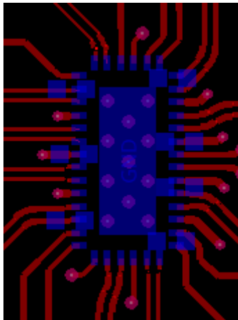
Figure 7-13. TMUXHS4446 Layout Example
