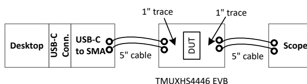
Figure 7-10. 10Gbps USB Compliance Setup - with TMUXHS4446
