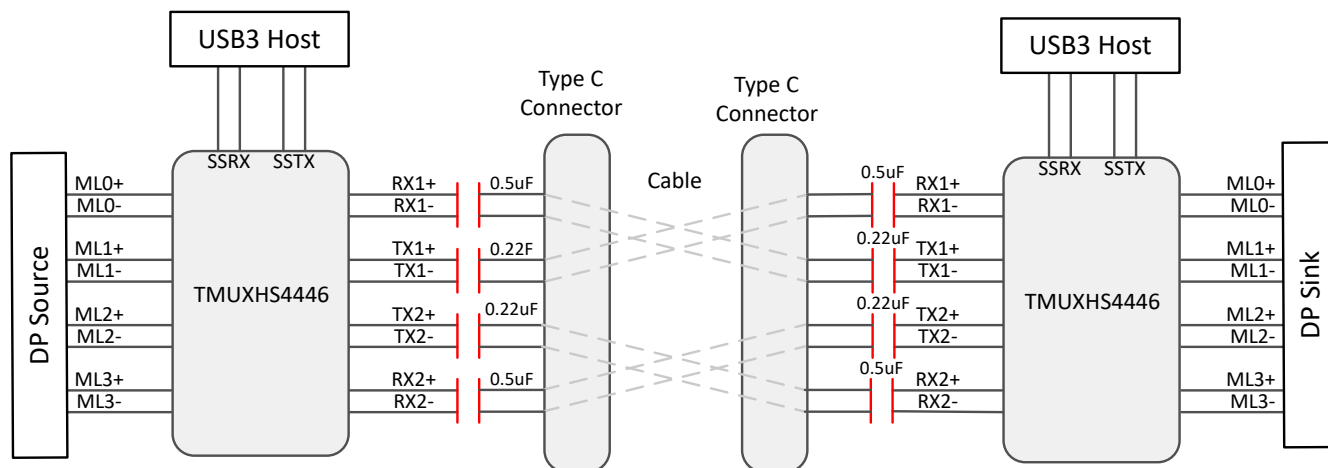
Figure 7-4. Placement of AC coupling Capacitors with V_{cm} > 1.8V
