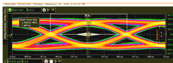
Figure 7-8. 8.1Gbps DP Compliance Eye Diagram - with TMUXHS4446
