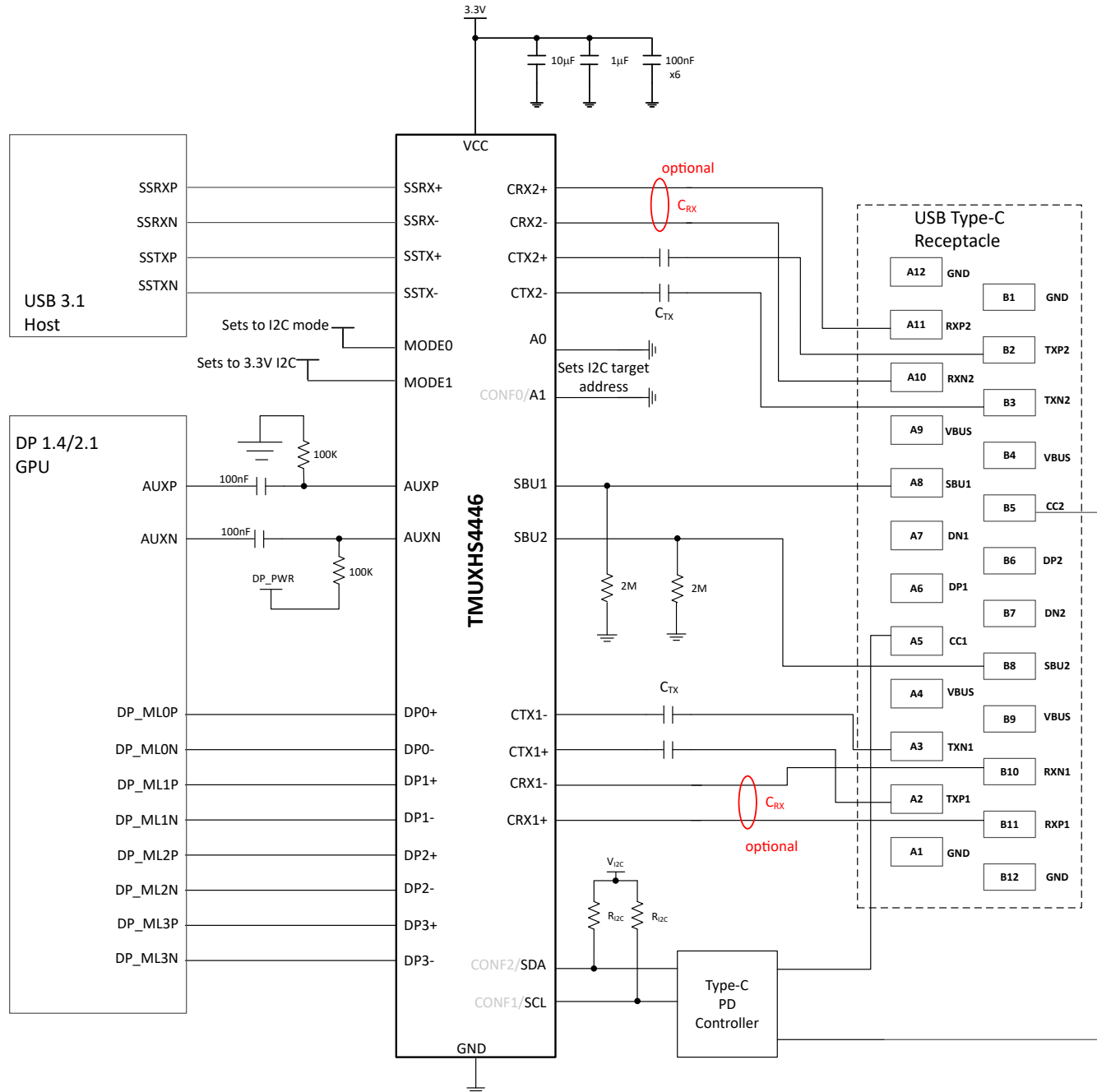
Figure 7-2. Application Schematic for TMUXHS446 in a Typical USB Type-C Source Use Case
