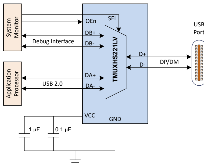
Figure 8-1. Routing Debug Signals to USB Port
