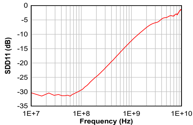
Figure 6-2. Typical Differential Return Loss vs Frequency
