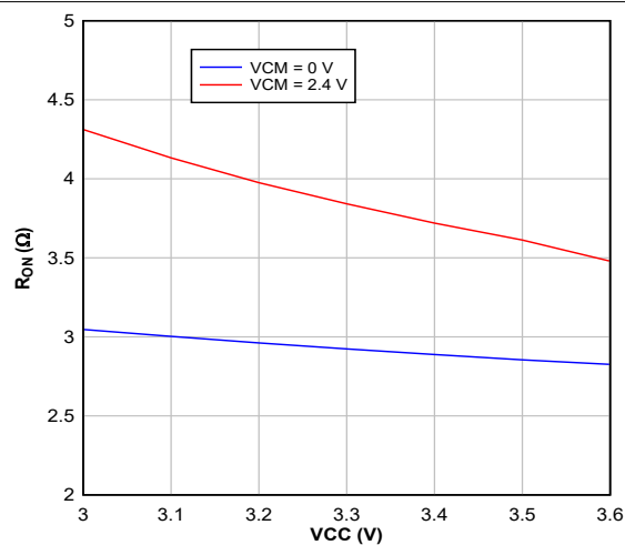
Figure 6-8. R_{ON} vs Supply Voltage VCC
