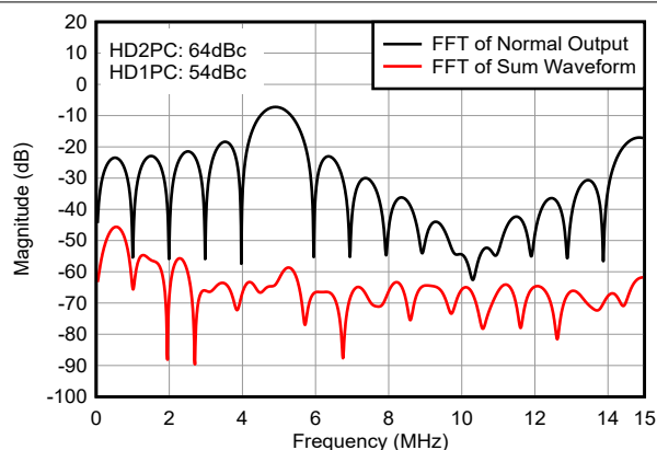
Figure 8-13. Pulser + TMUX9616, Mux Output Side, \pm 60V Pulser Supplies, 5MHz, 5 Cycles, 100\Omega \parallel 100pF Load
