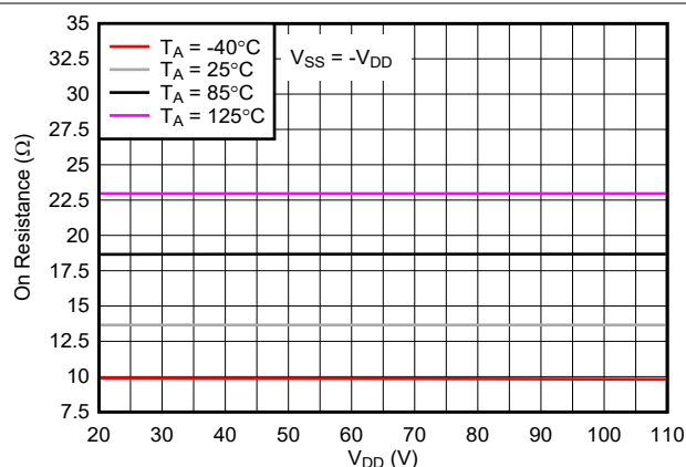
Figure 5-3. On-Resistance vs V_{DD}/V_{SS} Supply Voltage
