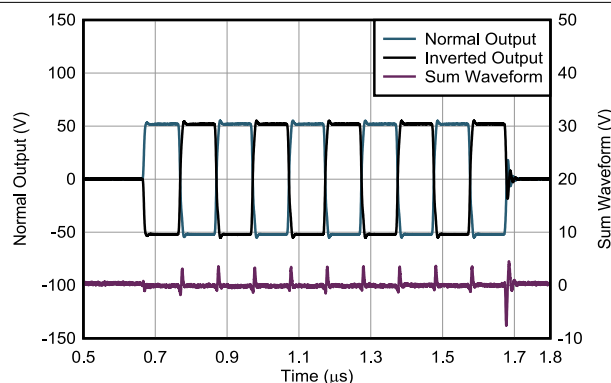
Figure 8-10. Pulser Only, Mux Output Side, \pm 60V Pulser Supplies, 5MHz, 5 Cycles, 100\Omega \parallel 100pF Load
