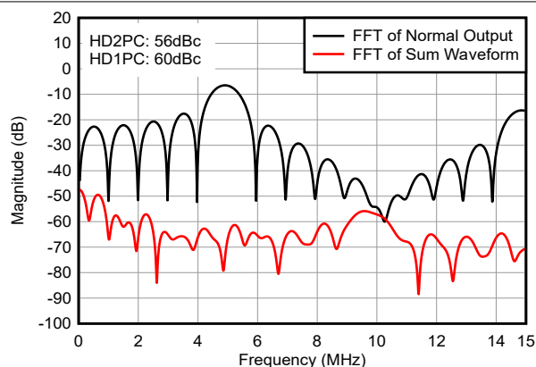
Figure 8-12. Pulser Only, Mux Output Side, \pm 60V Pulser Supplies, 5MHz, 5 Cycles, 100\Omega \parallel 100pF Load
