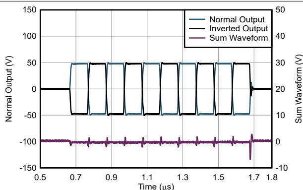
Figure 8-11. Pulser + TMUX9616, Mux Output Side, \pm 60V Pulser Supplies, 5MHz, 5 Cycles, 100\Omega \parallel 100pF Load
