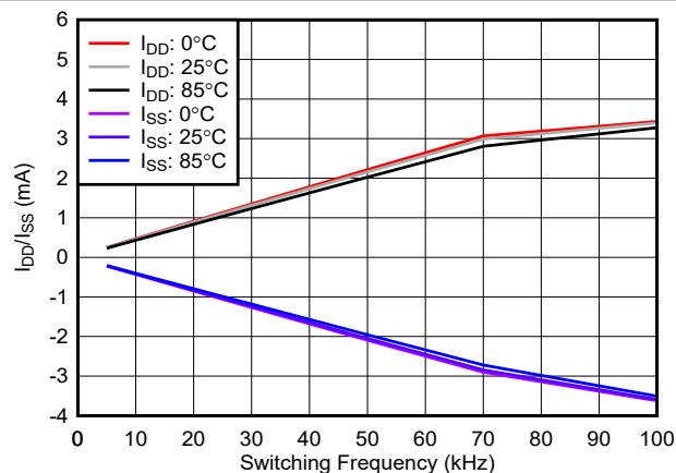
Figure 5-5. High Voltage Supply Current vs Switching Frequency
