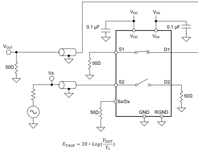
Figure 6-4. Crosstalk Measurement Setup
