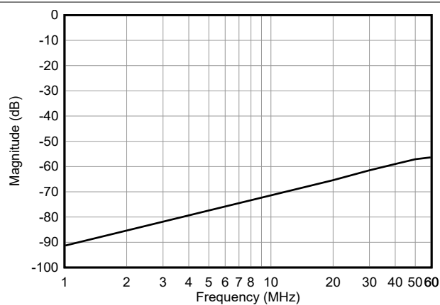
Figure 5-9. Large Signal Crosstalk vs Frequency
