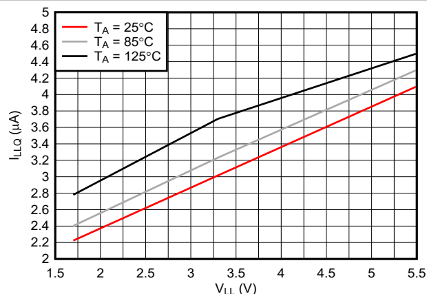
Figure 5-6. I_{LLQ} vs V_{LL}
