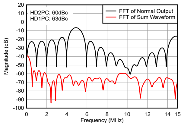
Figure 8-8. Pulser Only, Mux Input Side, \pm 60V Pulser Supplies, 5MHz, 5 Cycles, 100\Omega \parallel 100pF Load
