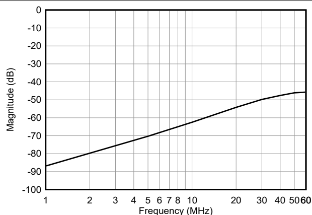
Figure 5-8. Large Signal Off Isolation vs Frequency
