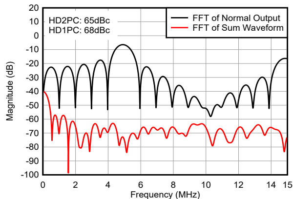
Figure 8-9. Pulser + TMUX9616, Mux Input Side, \pm 60V Pulser Supplies, 5MHz, 5 Cycles, 100\Omega \parallel 100pF Load
