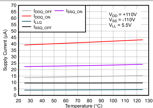
Figure 5-4. Supply Quiescent Current vs Temperature
