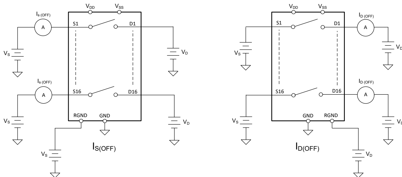
Figure 6-1. Off-Leakage Measurement Setup
