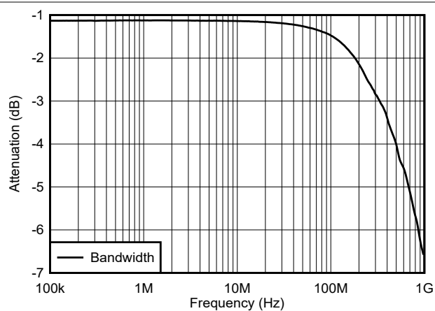
Figure 5-10. Small Signal Insertion Loss vs Frequency
