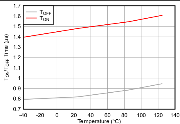
Figure 5-7. Turn ON and Turn OFF Time vs Temperature
