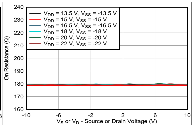
Figure 9-3. R_{ON} Flatness in Non-Fault Region
