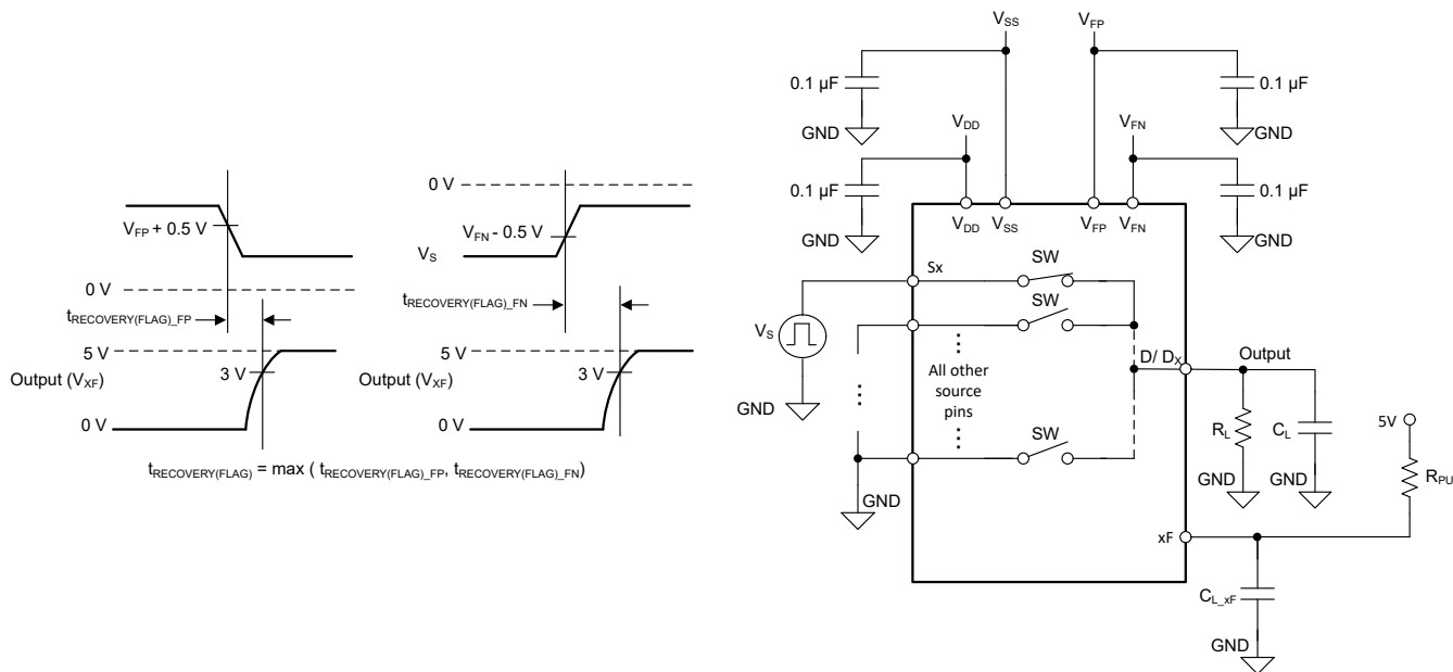
Figure 8-12. Fault Flag Recovery Time Measurement Setup
