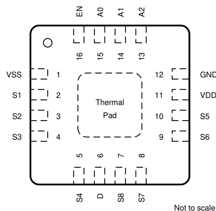
Figure 6-1. PW Package, 16-Pin TSSOP (Top View) Figure 6-2. RRP Package, 16-Pin WQFN (Top View)
