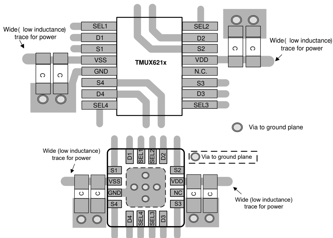
Figure 9-5. TMUX621x Layout Example
