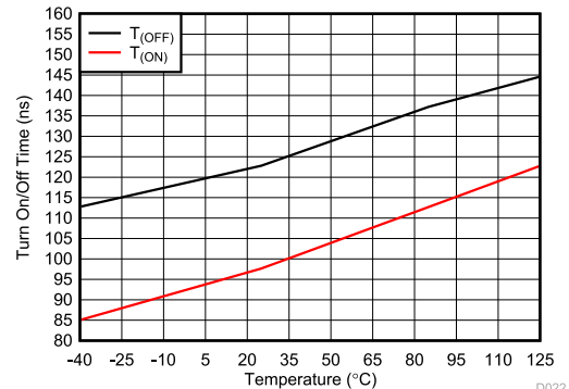
V_{DD} = 15\text{ V}, V_{SS} = -15\text{ V} Figure 6-18. T_{ON} and T_{OFF} vs Temperature
