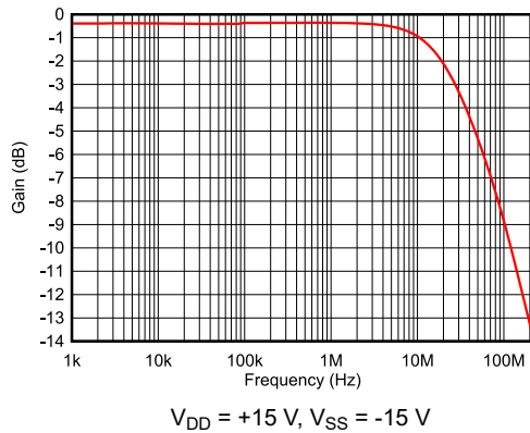
Figure 6-25. On Response vs Frequency
