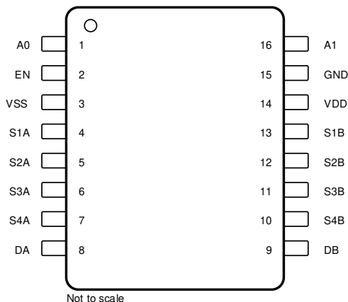
Figure 5-3. TMUX6209: PW Package 16-Pin TSSOP Top View
