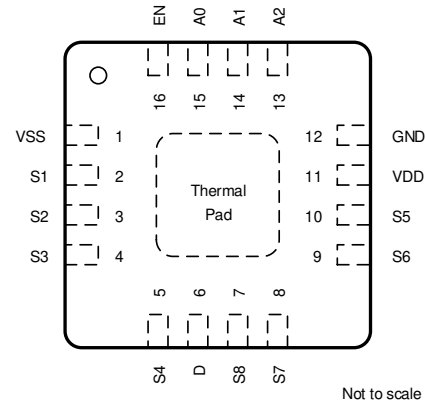
Figure 5-2. TMUX6208: RUM Package 16-Pin WQFN Top View
