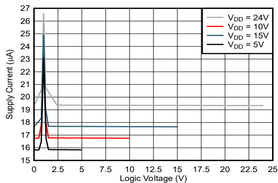
Figure 6-4. Supply Current vs Logic Voltage
