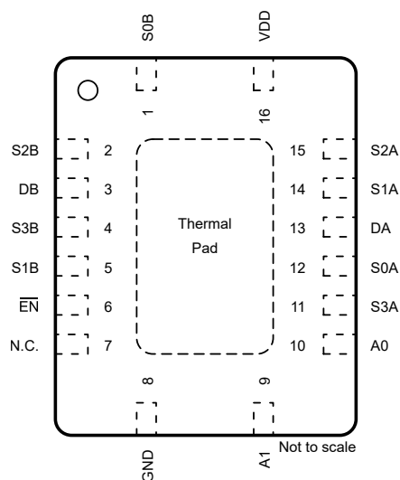
Figure 6-6. TMUX1309-Q1: BQB Package, 16-Pin WQFN (Top View)
