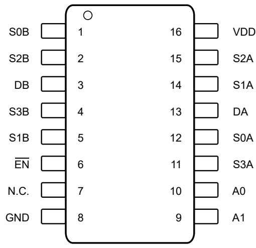
Figure 6-5. TMUX1309-Q1: DYY Package, 16-Pin SOT-23-THIN (Top View)
