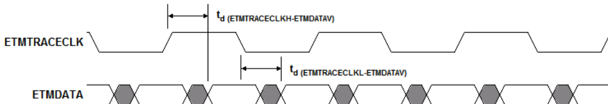
Figure 6-25. ETMDATA Timing
