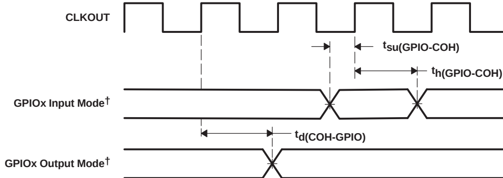
Figure 5-31. \text{GPIOx}^\dagger Timings
