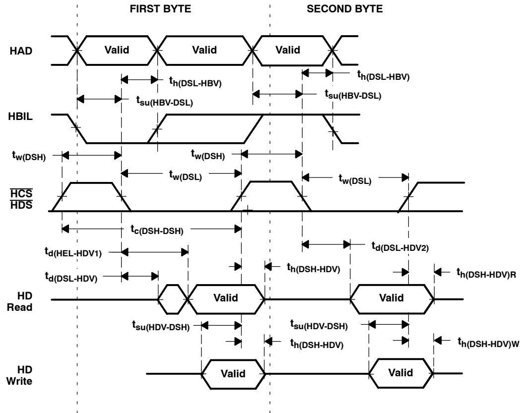
Figure 29. Read/Write Access Timings Without HRDY or \overline{HAS}
