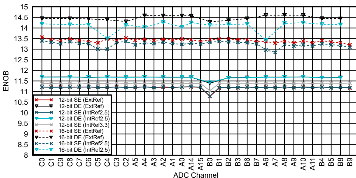
Figure 6-54. Per-Channel ENOB for 169-Ball NMR
