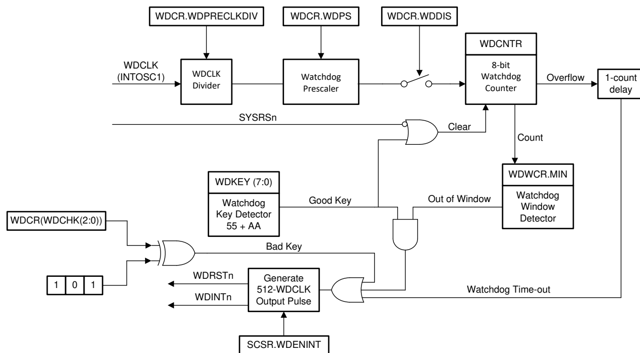
Figure 7-7. Windowed Watchdog
