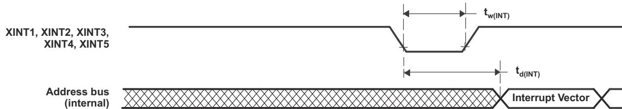
Figure 6-37. External Interrupt Timing
