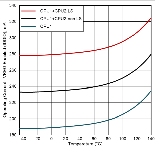
Figure 6-2. Typical Operating Current Versus Temperature - VREG Enabled
