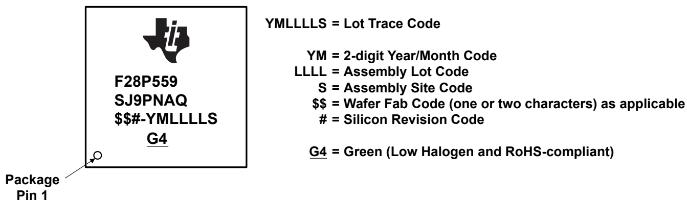
Figure 9-5. Package Symbolization for PNA Package – Automotive
