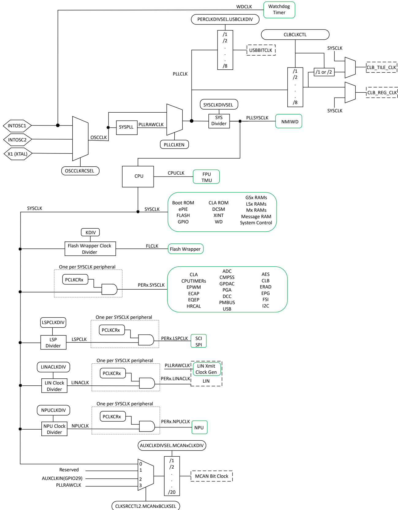
Figure 6-9. Clocking System
