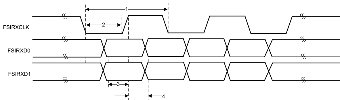
Figure 6-80. FSIRX Timings
