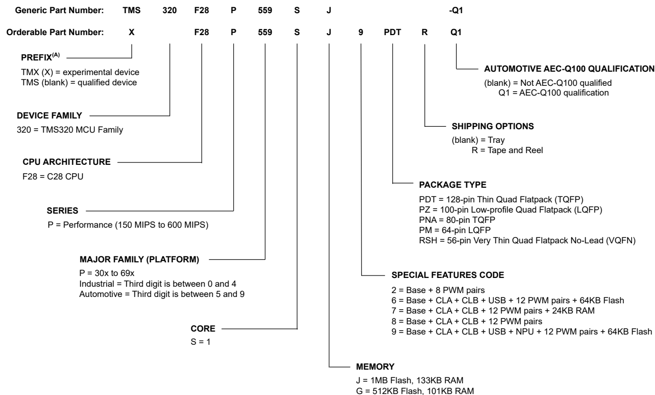
Figure 9-1. Device Nomenclature
