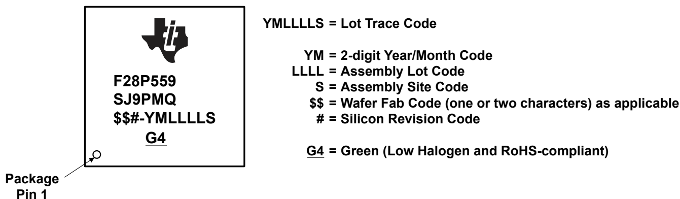
Figure 9-7. Package Symbolization for PM Package – Automotive
