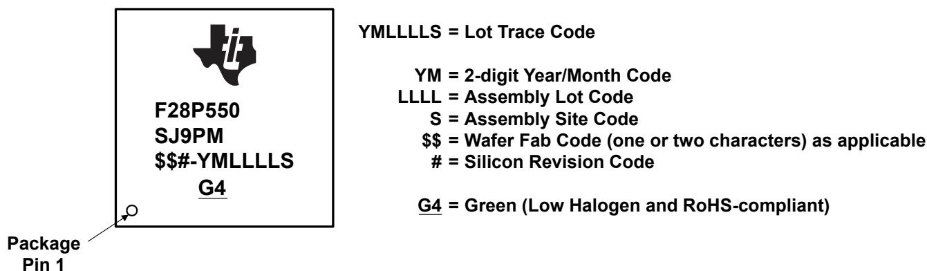
Figure 9-8. Package Symbolization for PM Package – Non-Automotive
