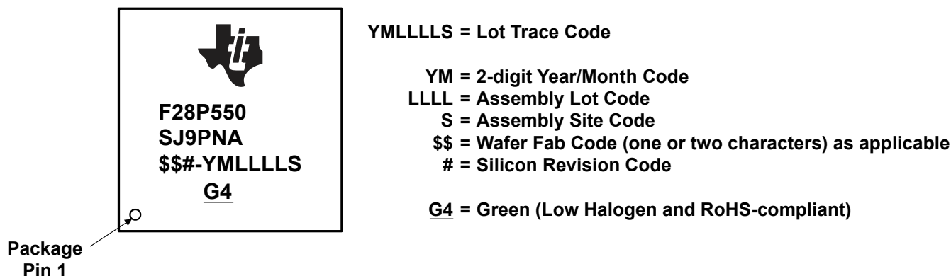
Figure 9-6. Package Symbolization for PNA Package – Non-Automotive
