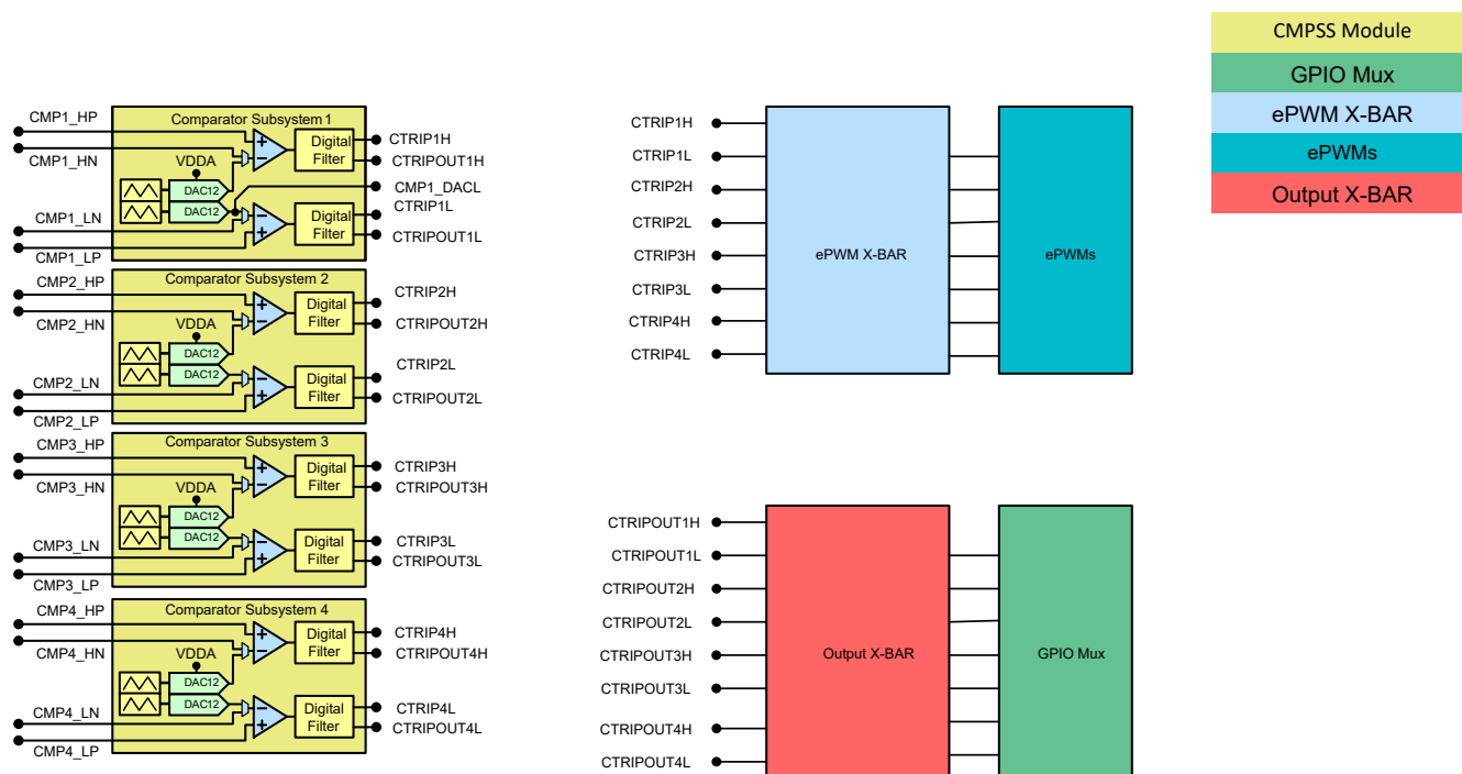
Figure 6-46. CMPSS Connectivity
