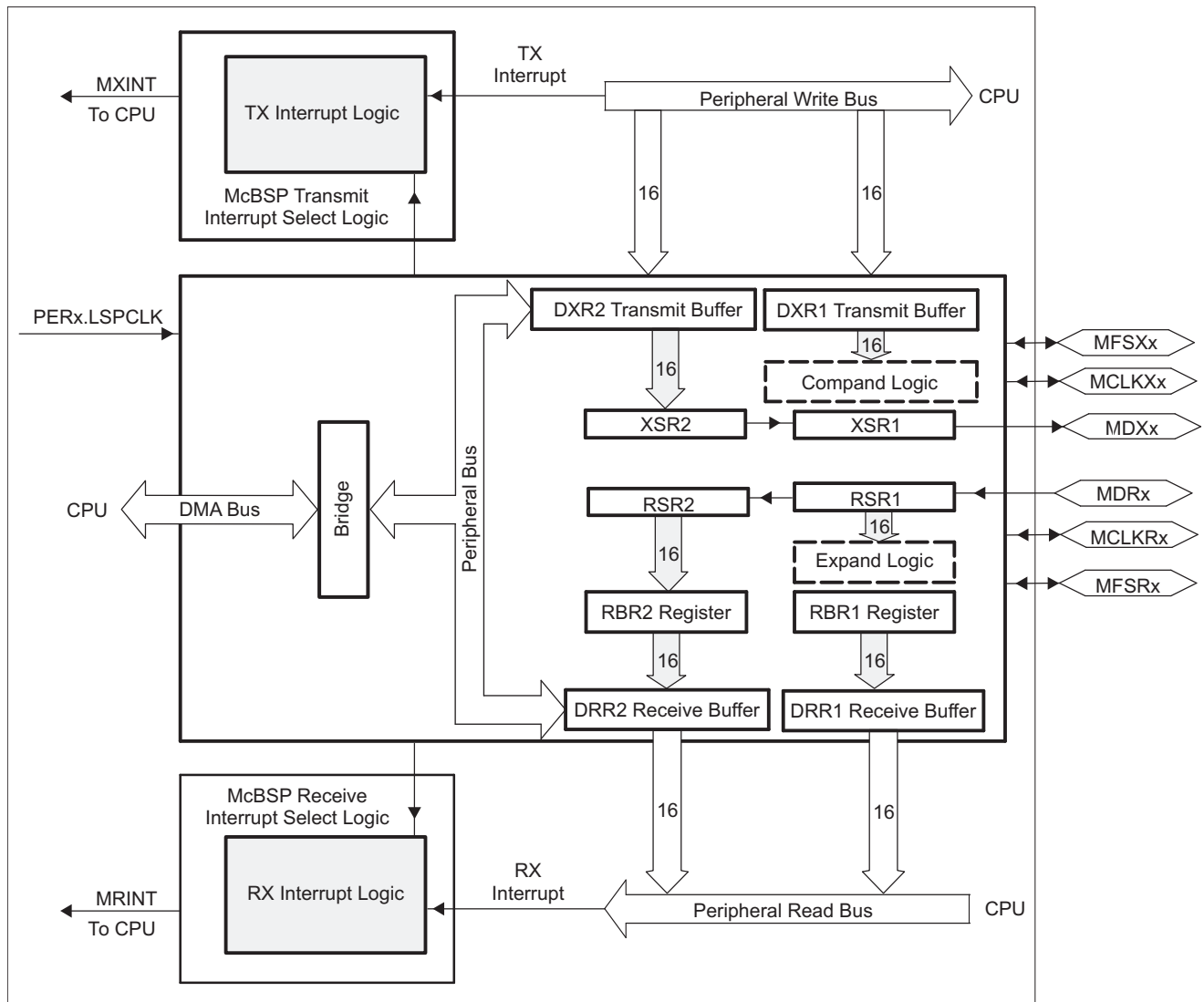
Figure 4-60. McBSP Block Diagram
