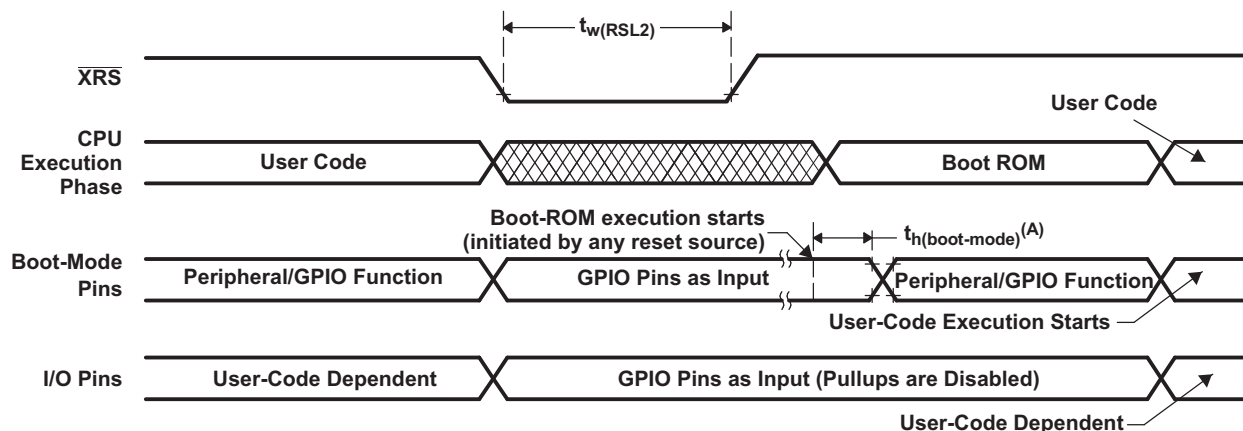
Figure 4-6. Power-on Reset
