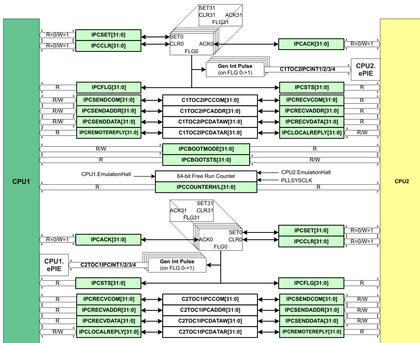
Figure 5-4. IPC Architecture
