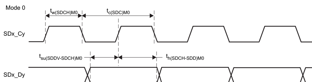
Figure 4-55. SDFM Timing Diagram – Mode 0
