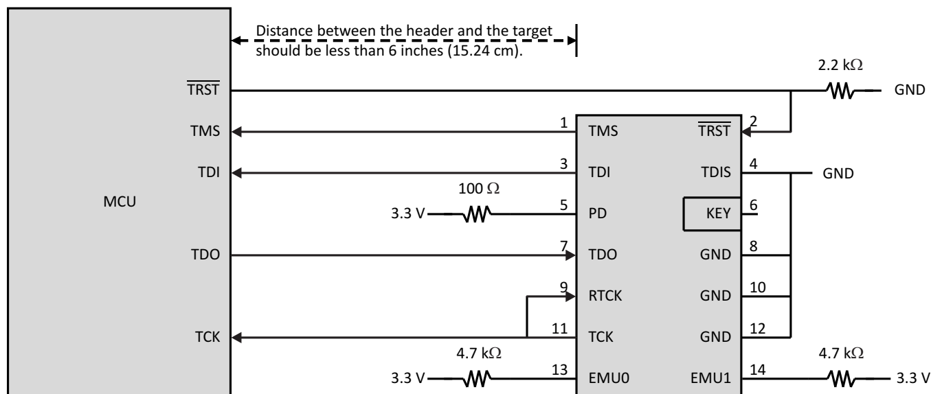
Figure 4-10. Connecting to the 14-Pin JTAG Header
