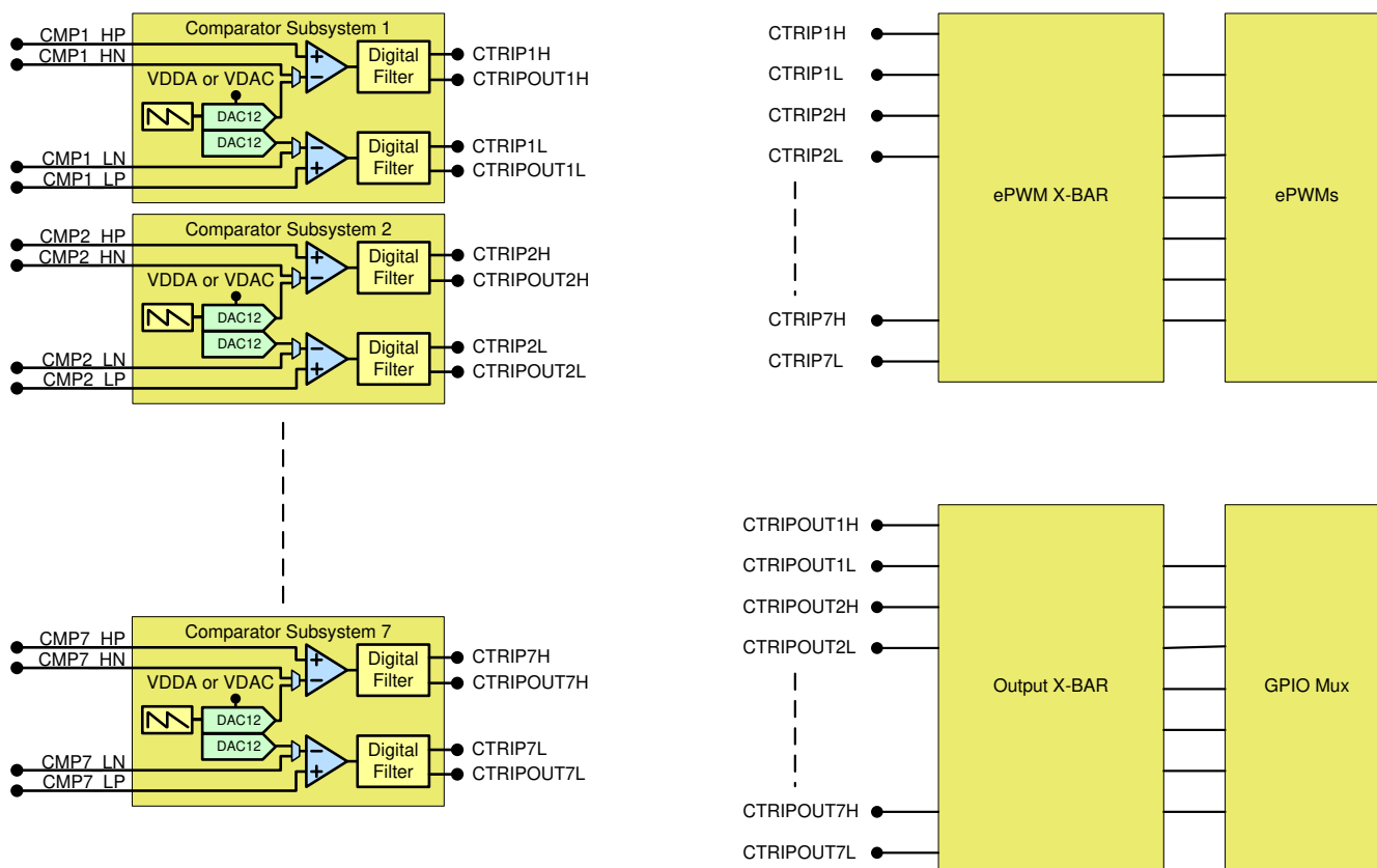
Figure 7-57. CMPSS Connectivity
