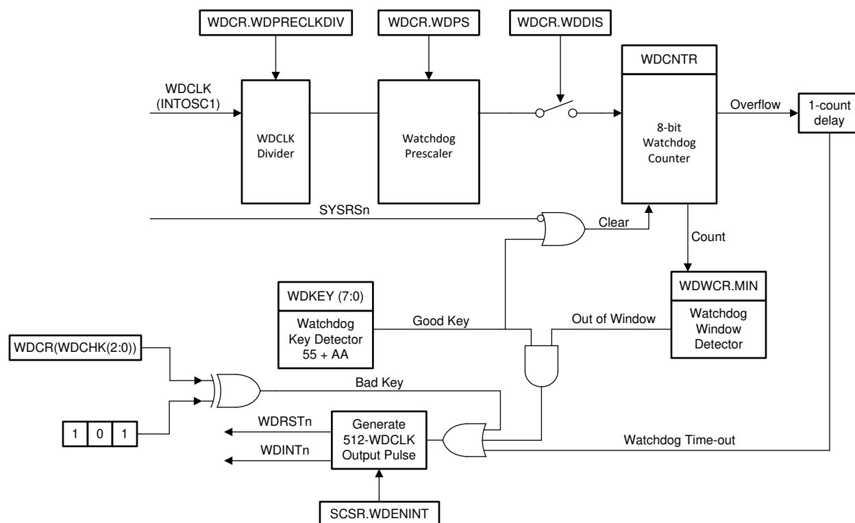
Figure 7-3. Windowed Watchdog
