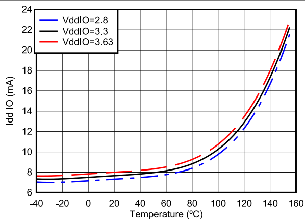
Figure 6-5. Current Versus Temperature – STANDBY Mode
