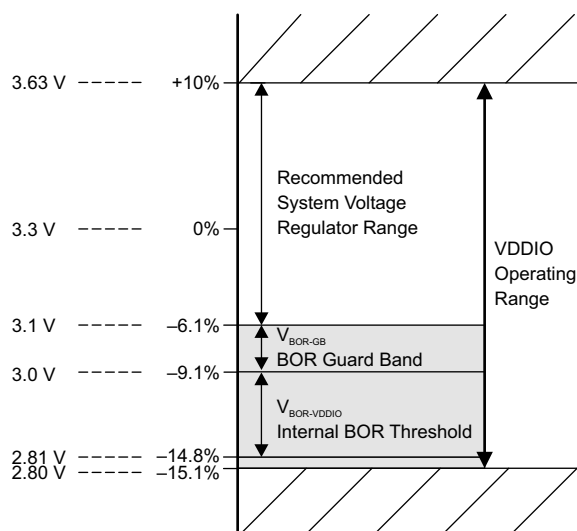
Figure 6-8. I/O BOR Operating Region
