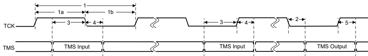
Figure 6-25. cJTAG Timing
