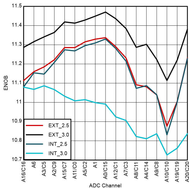
Figure 6-42. Per-Channel ENOB for 48-Pin PT LQFP
