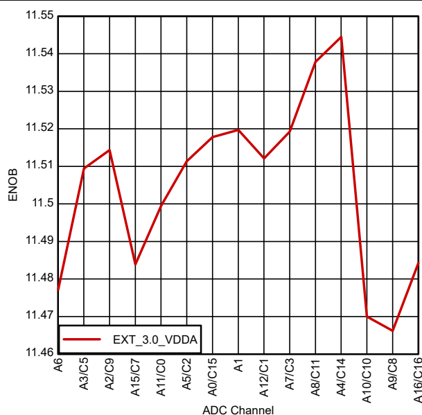
Figure 6-44. Per-Channel ENOB for 32-Pin RHB VQFN
