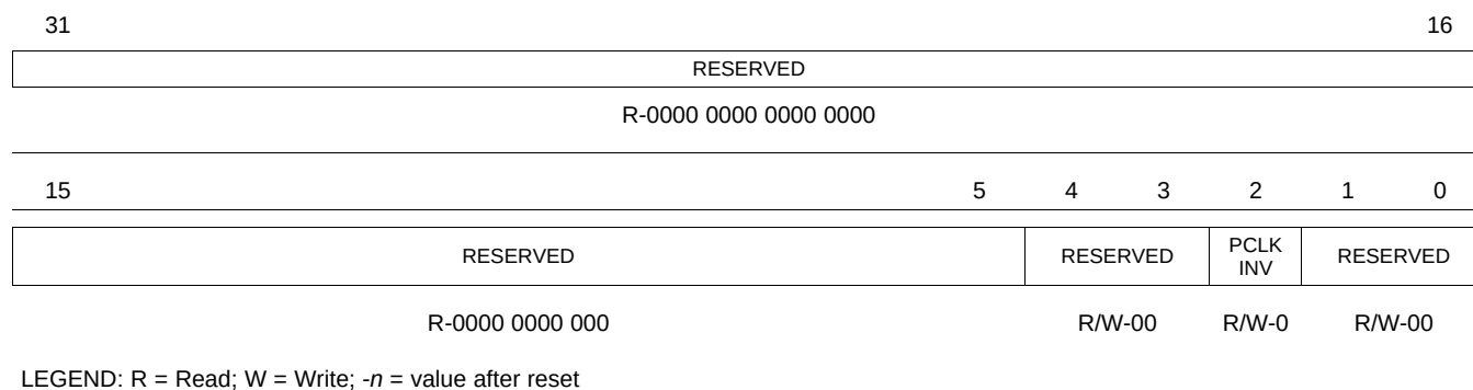
Figure 3-2. VPSS_CLKCTL Register
