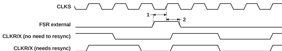
Figure 6-28. FSR Timing When GSYNC = 1
