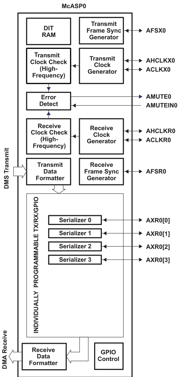
Figure 6-33. McASP0 Configuration
