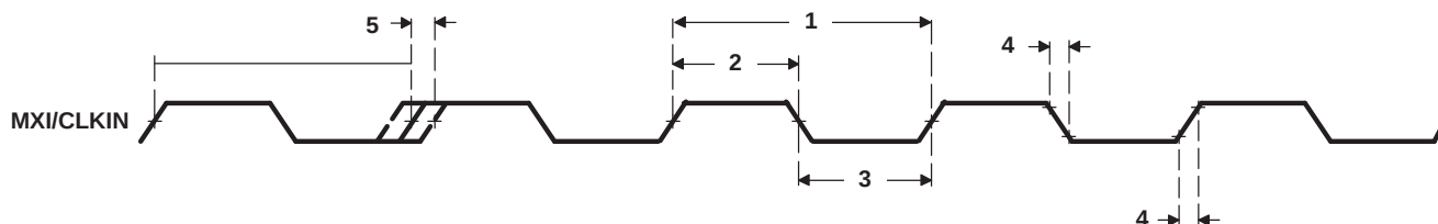
Figure 6-13. MXI/CLKIN Timing
