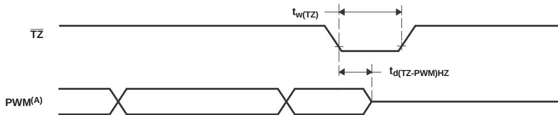
Figure 6-48. PWM Hi-Z Characteristics
