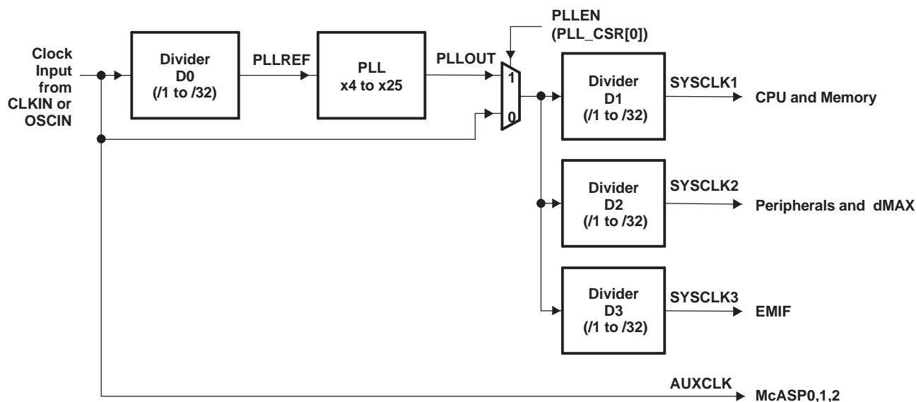
Figure 4-43. PLL Topology
