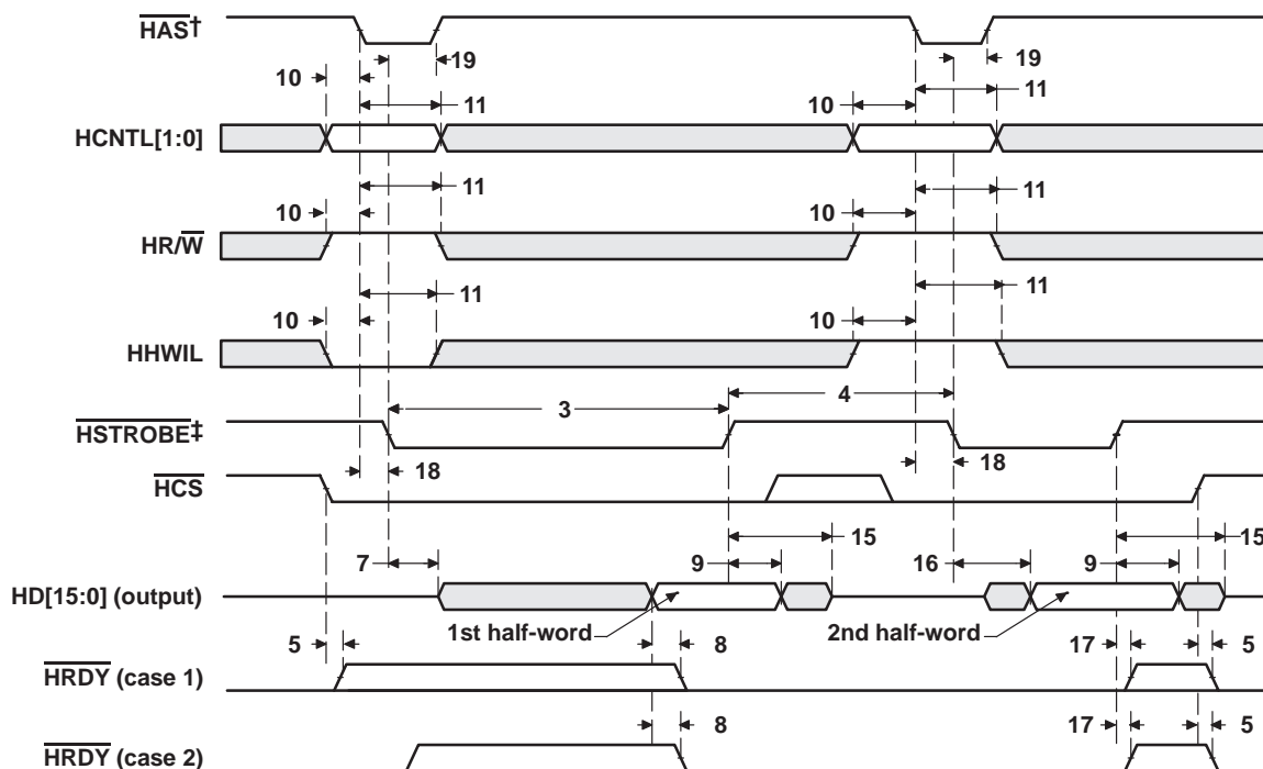
Figure 43. HPI Read Timing ( \overline{HAS} Used)
