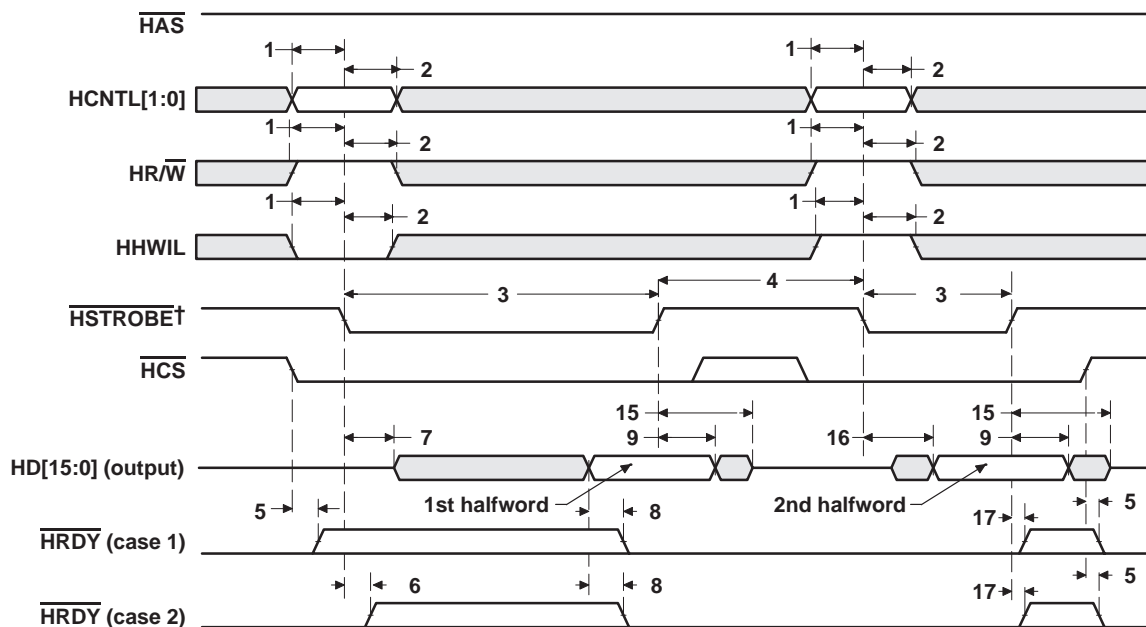
Figure 42. HPI Read Timing ( \overline{HAS} Not Used, Tied High)
