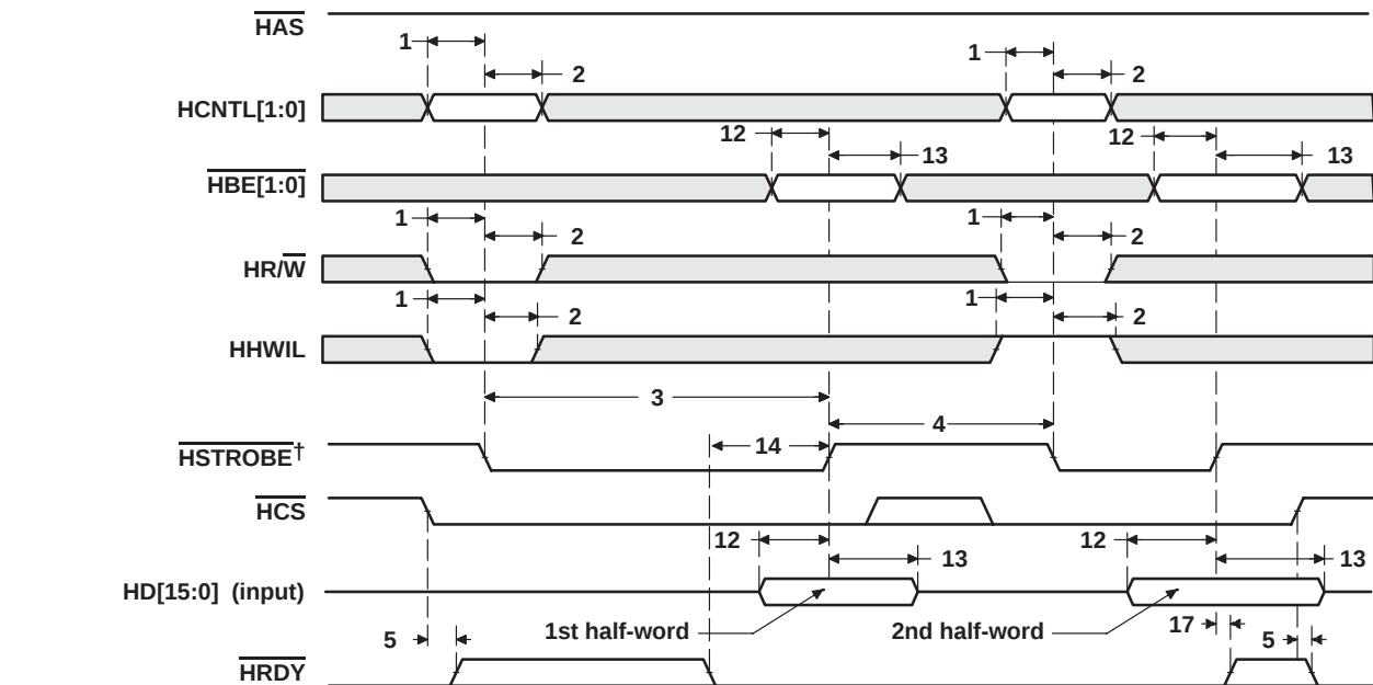
Figure 31. HPI Write Timing ( \overline{HAS} Not Used, Tied High)
