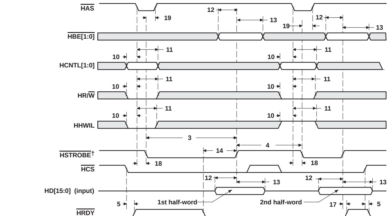
Figure 32. HPI Write Timing ( \overline{HAS} Used)
