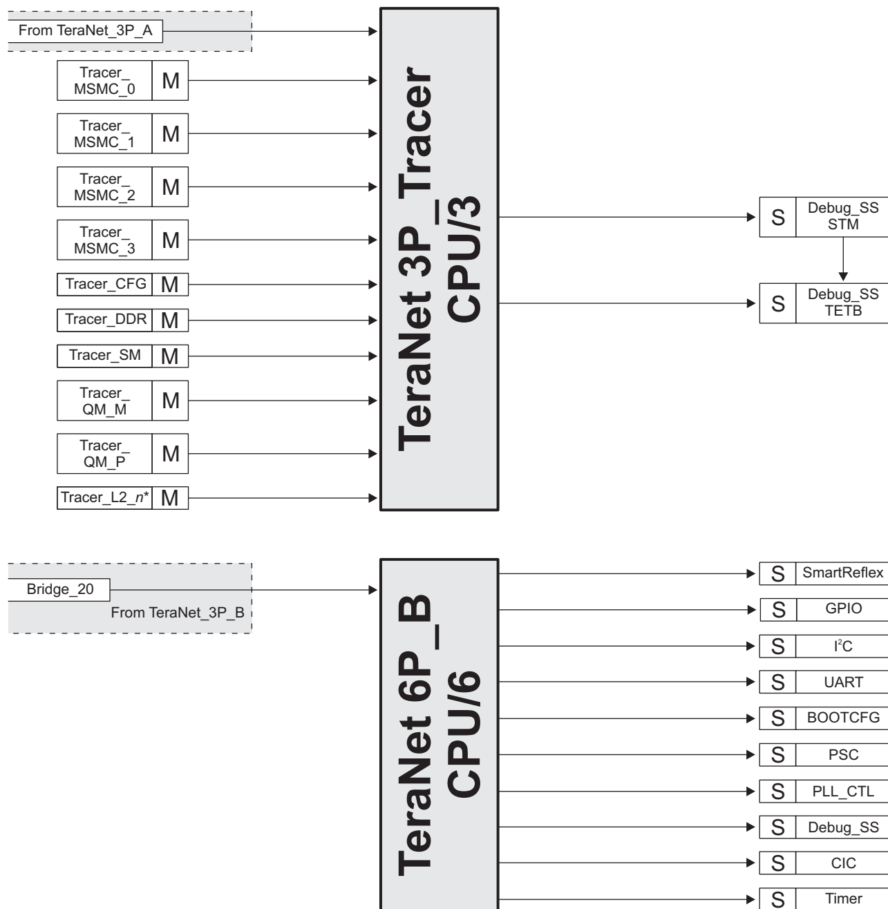
Figure 4-4 TeraNet 6P_B and 3P_Tracer for C6674
