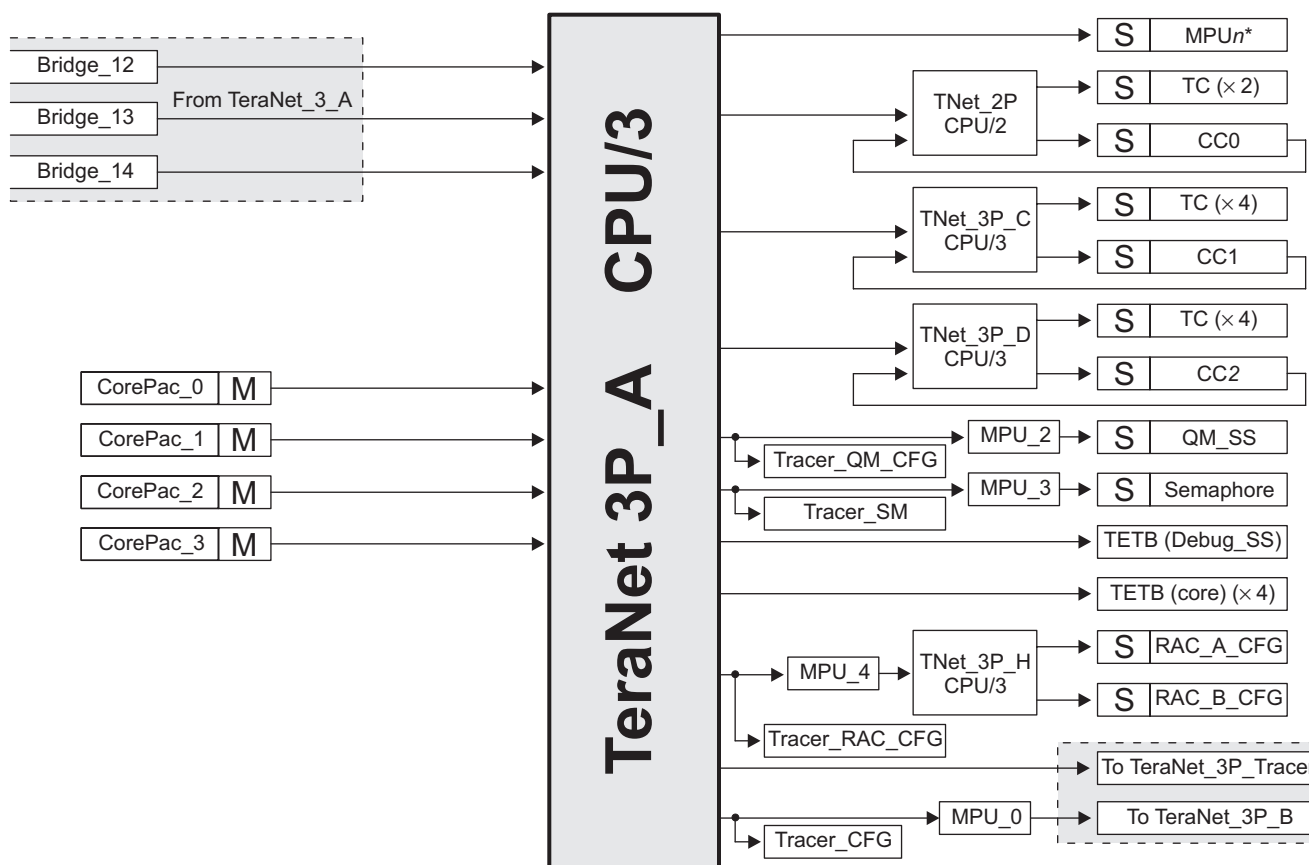
Figure 4-4 TeraNet 3P_A
