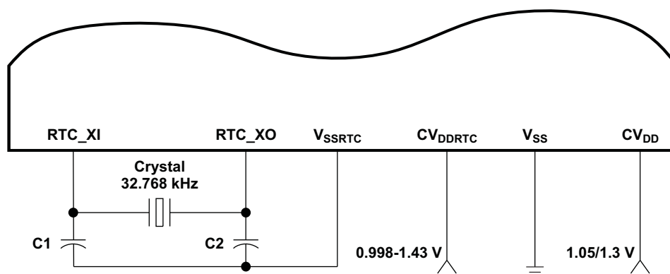
Figure 5-11. 32.768-kHz RTC Oscillator
