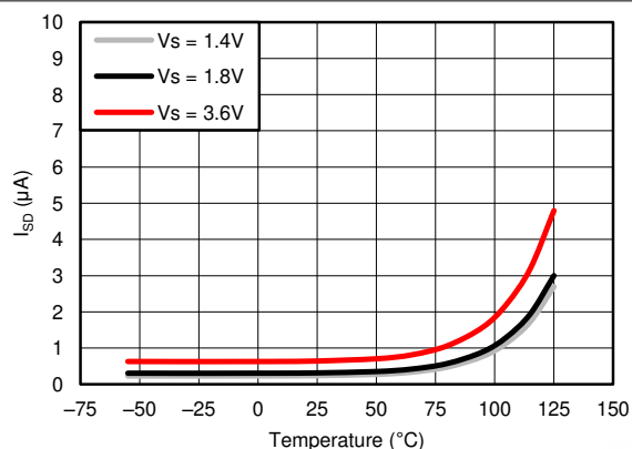
Figure 6-2. Shutdown Current vs Temperature
