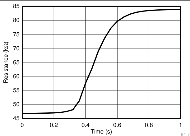
Figure 7-8. DEC Thermal Response Time
