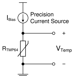
Figure 9-3. TMP64 Biasing Circuit With Current Source
