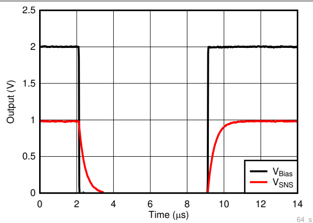
Figure 7-7. Step Response
