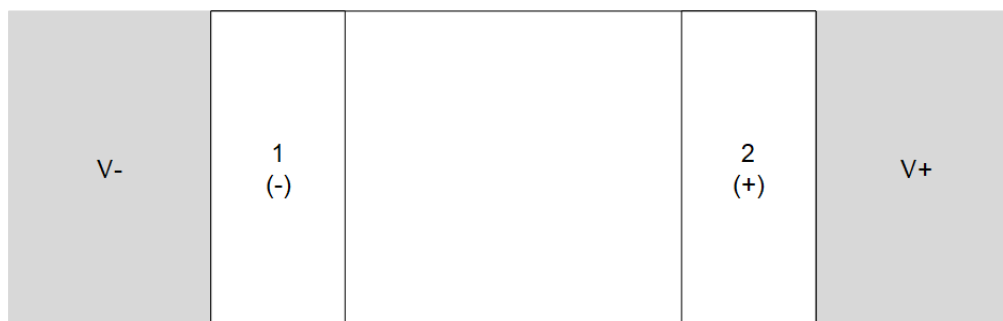
Figure 10-1. DEC Package Recommended Layout
