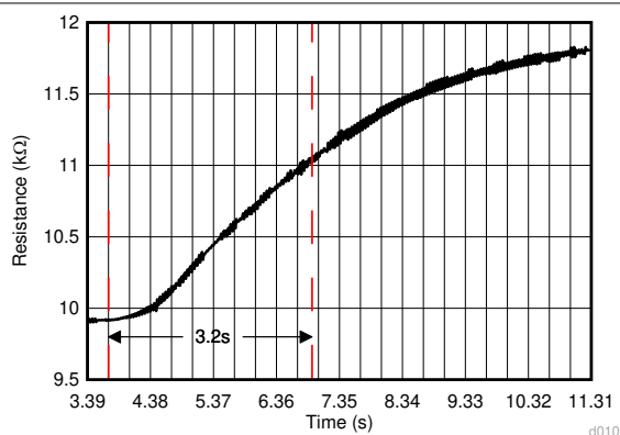
Figure 6-7. Step Response
