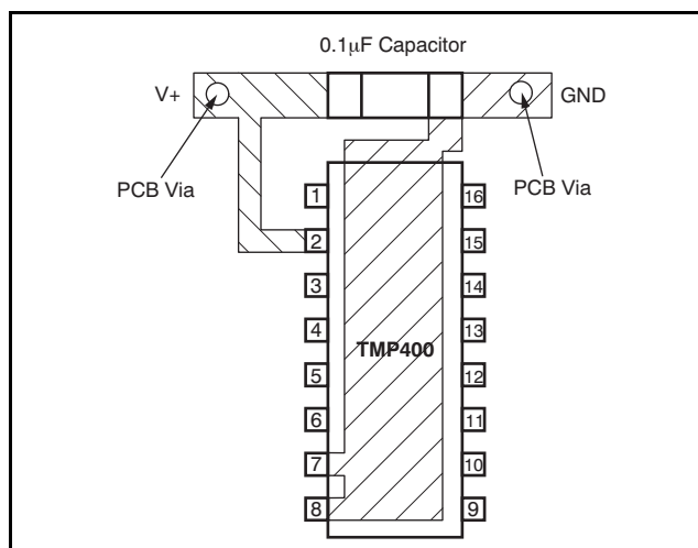
Figure 20. Suggested Bypass Capacitor Placement
