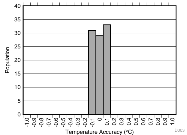
Typical Trip Threshold Accuracy at -20^\circ\text{C} to 125^\circ\text{C}
