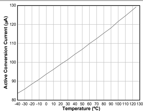
Figure 6-9. Active Conversion Current vs Temperature
