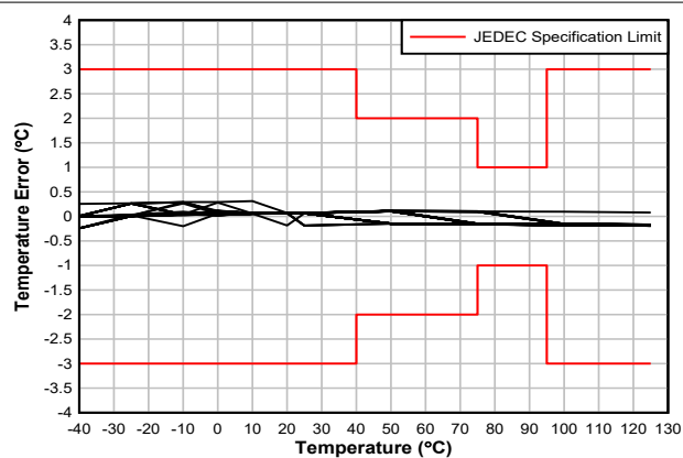
Figure 6-8. Temperature Error vs Temperature
