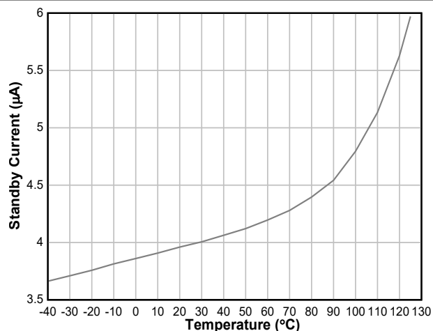
Figure 6-11. Standby Current vs Temperature
