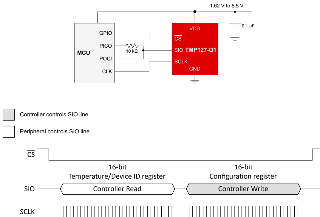
Figure 9-2. 4-Wire Configuration
