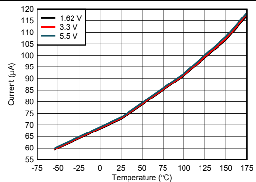
Figure 7-3. Active Conversion Current vs. Temperature
