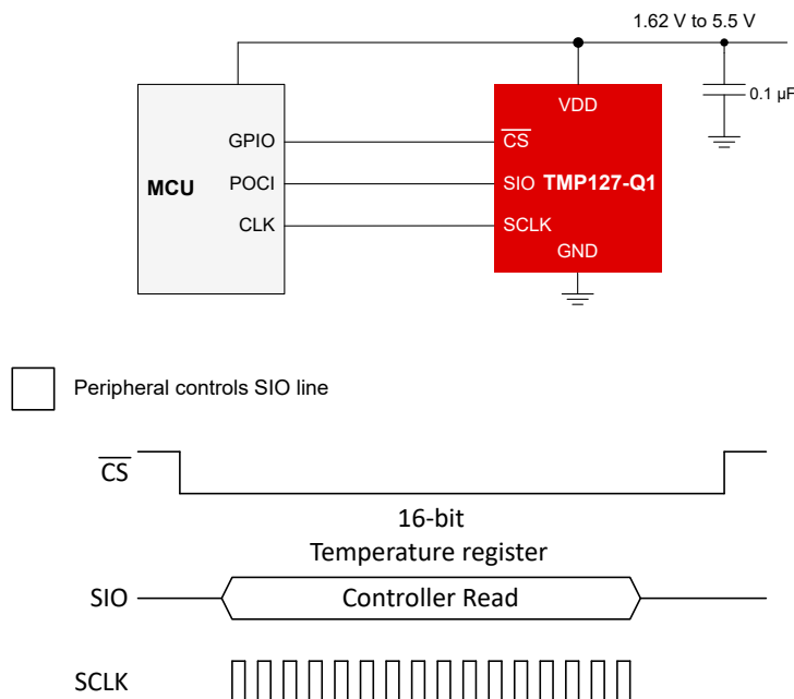
Figure 9-1. Read-Only Configuration
