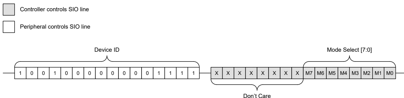
Figure 8-3. Shutdown Mode SPI Communication
