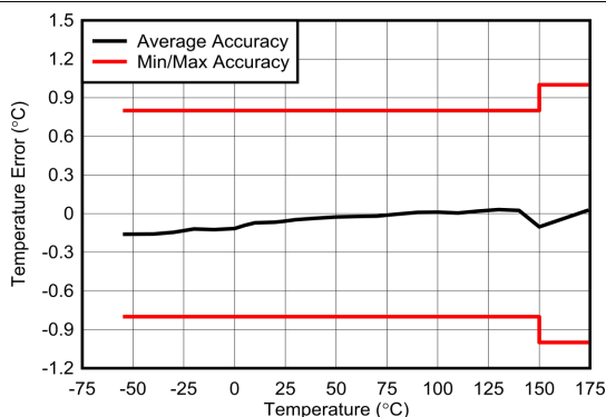
Figure 7-2. Temperature Accuracy
