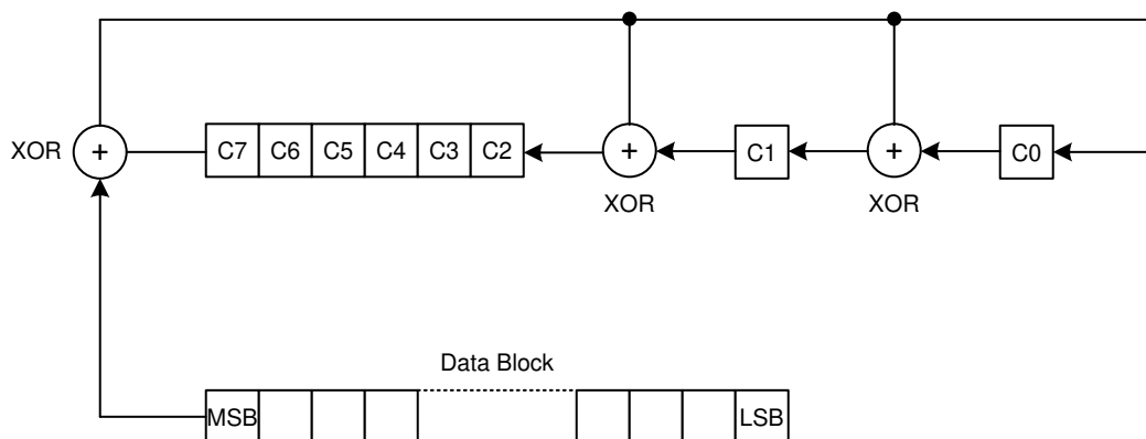
Figure 8-19. CRC Module
