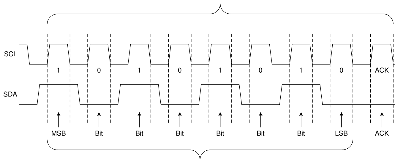
Figure 8-8. Bit Transfer
