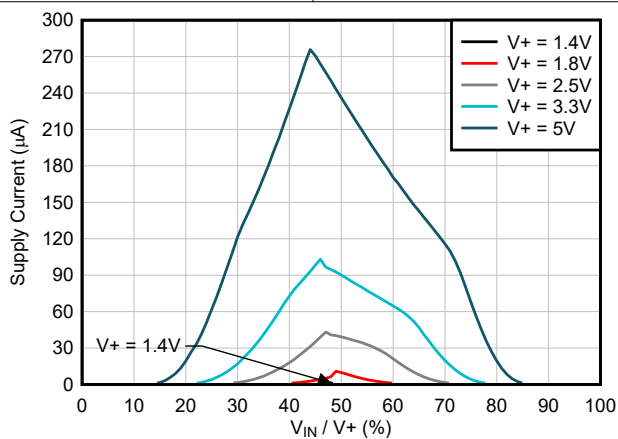
Figure 6-16. Supply Current vs one Input Cell Input Voltage
