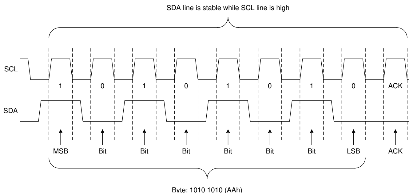
Figure 7-6. Bit Transfer
