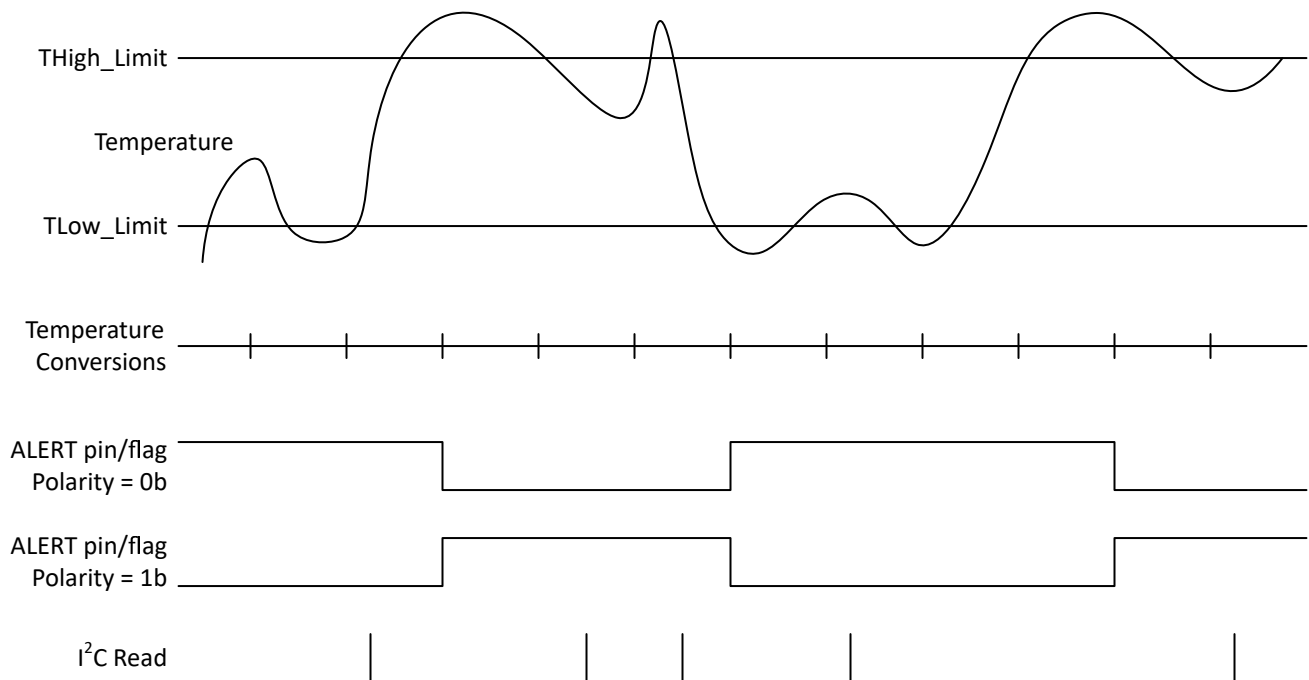
Figure 7-1. Comparator Mode
