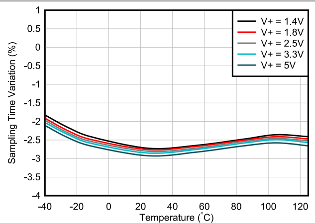
Figure 6-13. Sampling Time vs Temperature
