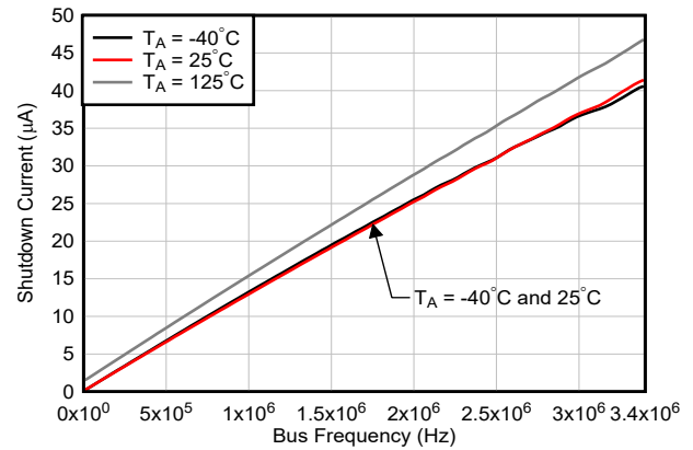
Figure 6-9. Shutdown Current vs Bus Frequency (Temperature at 3.3V Supply)
