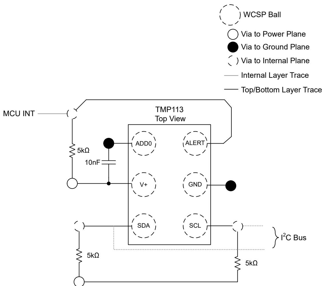
Figure 9-3. Layout Example
