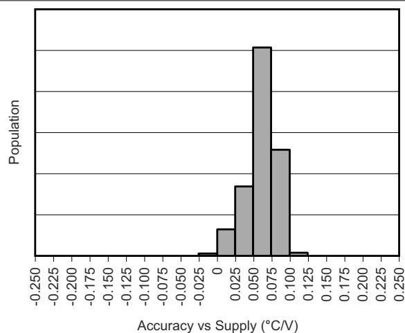
Figure 6-3. Accuracy vs. Supply
