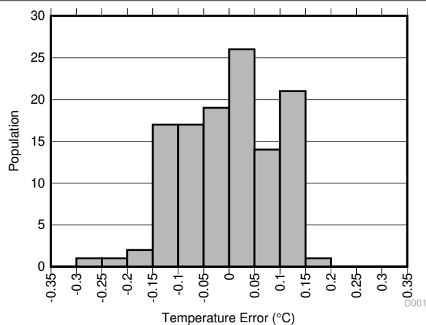
Figure 6-2. Temperature Error at 25°C
