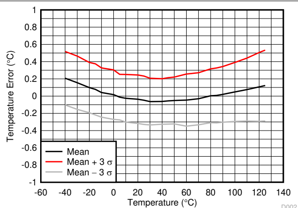
Figure 6-2. Temperature Error at 25°C
