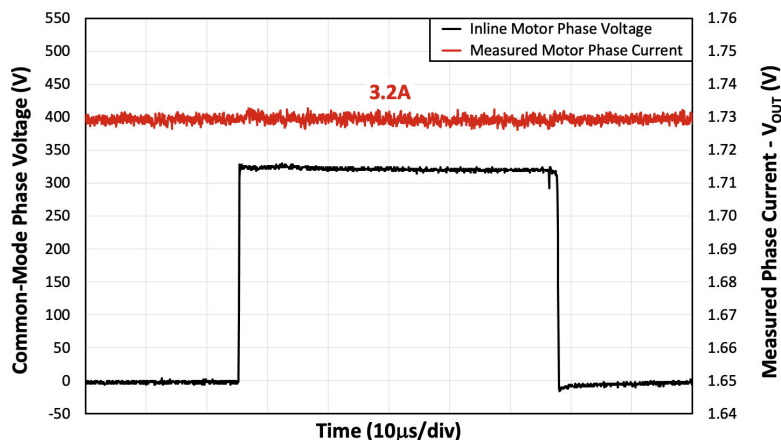
Figure 10-3. Inline Motor Current-Sense Input and Output Signals
