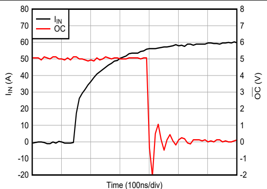
Figure 7-9. Overcurrent Output Response
