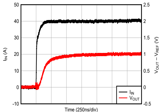
Figure 7-7. Voltage Output Step Response, Rising
