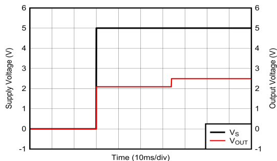
Figure 7-11. Startup Transient Response
