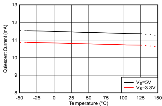
Figure 7-13. Quiescent Current vs Temperature
