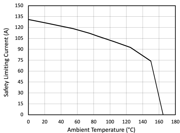
Figure 7-16. Thermal Derating Curve for Safety-Limiting Current, Side 1
