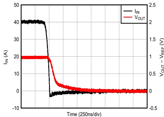
Figure 7-8. Voltage Output Step Response, Falling
