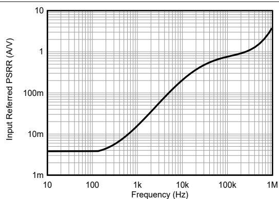
Figure 7-5. PSRR vs Frequency
