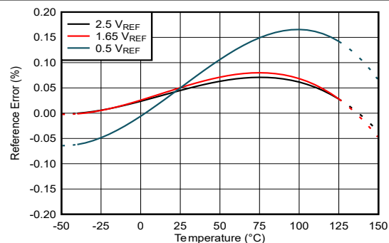
Figure 7-2. Reference Error vs Temperature
