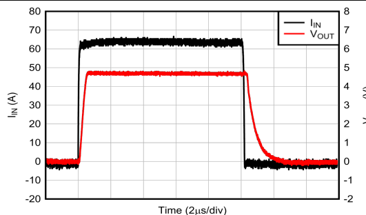
Figure 7-10. Current Overload Response
