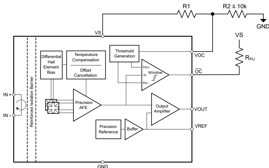
Figure 9-3. User Configurable Overcurrent Threshold Using Power Supply Voltage
