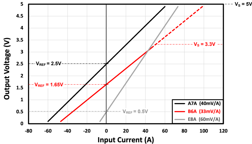
Figure 9-2. Output Voltage Relationship to Input Current for TMCS1148xxA
