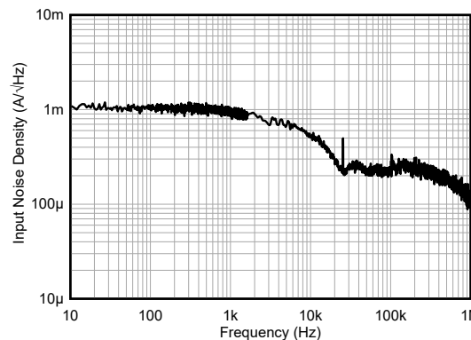
Figure 7-14. Input-Referred Noise Density vs Frequency
