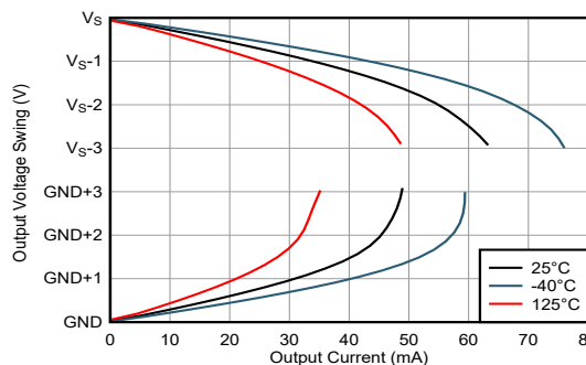
Figure 7-12. Output Swing vs Output Current
