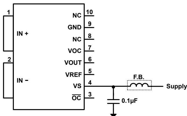
Figure 10-4. Power Supply Noise Filtering
