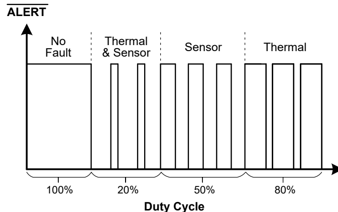
Figure 8-10. Sensor Diagnostics Waveform
