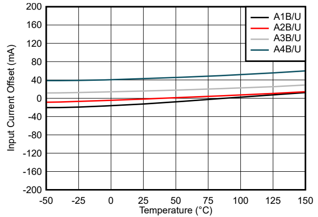
Figure 7-2. TMCS1108-Q1 Input Offset Current vs. Temperature
