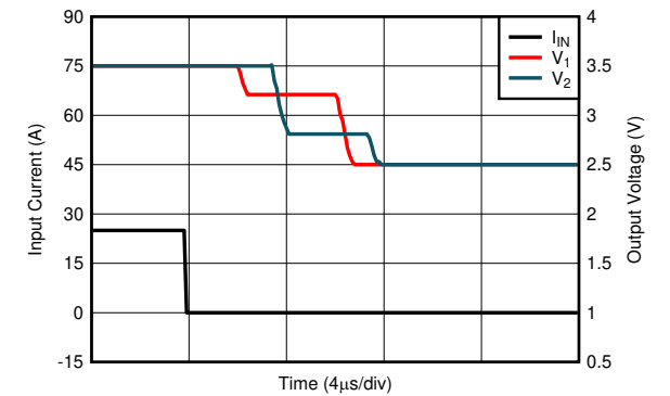
Figure 6-18. Voltage Output Step, Falling
